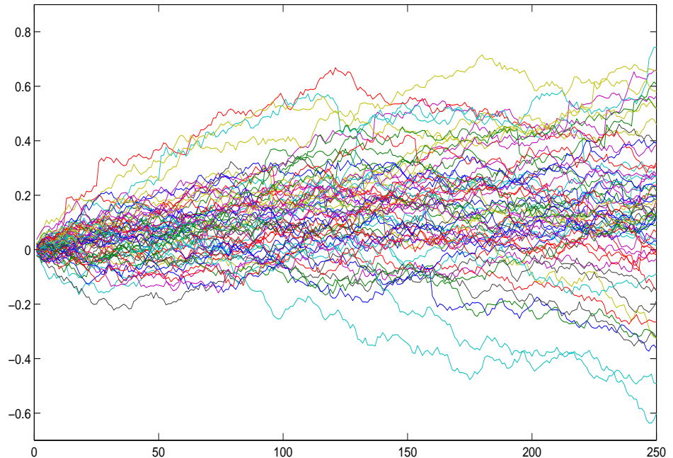
Figure 1: Simulation of trajectories with Clayton temporal dependence ( \tau = 0.1 ) and Normal distribution of increments with volatility equal to 0.2
