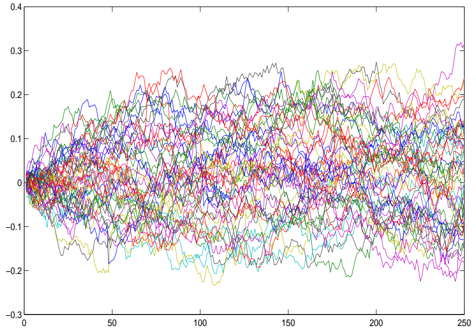
Figure 2: Simulation of martingale trajectories with Clayton temporal dependence ( \tau = 0.1 ) and Normal distribution of increments with volatility equal to 0.2
